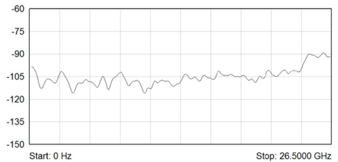
Typical Isolation (dB) - 26.5 GHz Underterminated Versions
