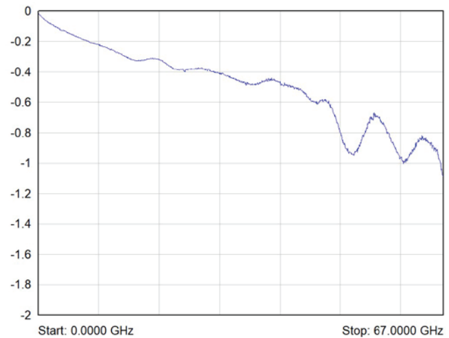
Typical Insertion Loss (dB) - 67 GHz Underterminated Versions
