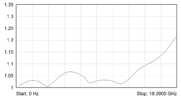
Typical VSWR - 18 GHz Underterminated Versions
