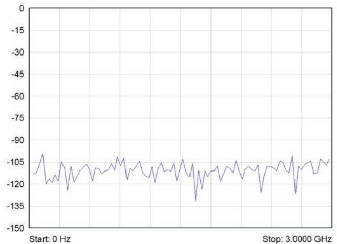
Typical Isolation (dB) - 3 GHz Terminated & Unterminated Versions
