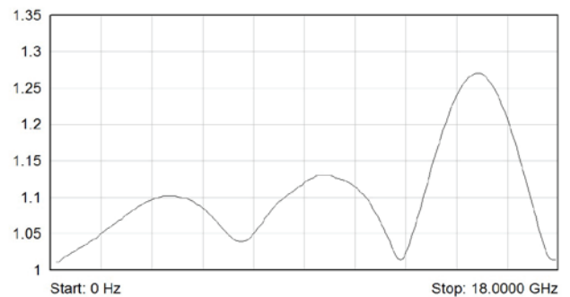
Typical VSWR - 18 GHz Terminated Versions
