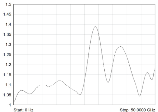
Typical VSWR - 50 GHz Terminated & Unterminated Versions
