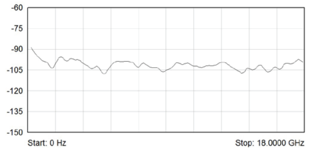
Typical Isolation (dB) - 18 GHz Terminated Versions
