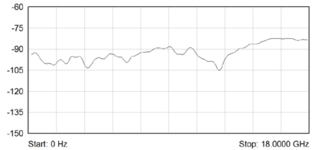
Typical Isolation (dB) - 18 GHz Underterminated Versions
