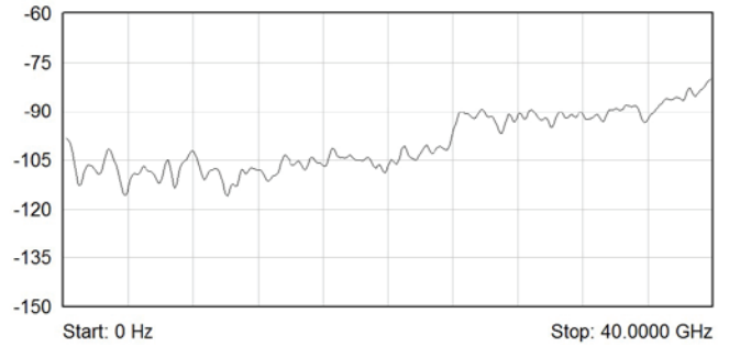
Typical Isolation (dB) - 40 GHz Unterminated Versions
