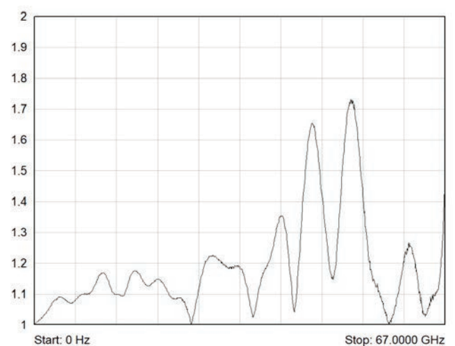
Typical VSWR - 67 GHz Terminated Versions
