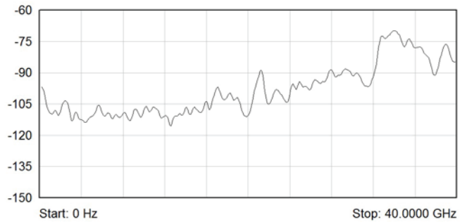
Typical Isolation (dB) - 40 GHz Terminated Versions
