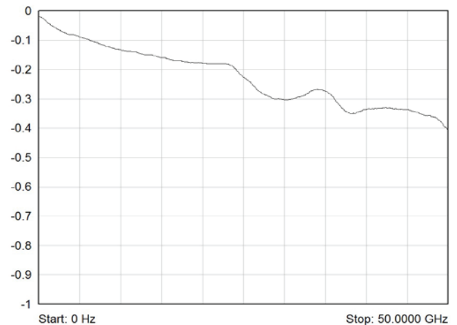
Typical Insertion Loss (dB) - 50 GHz Terminated & Unterminated Versions
