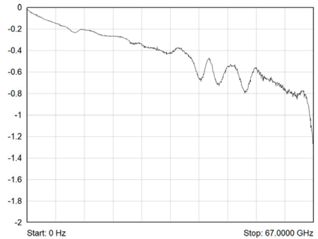
Typical Insertion Loss (dB) - 67 GHz Terminated Versions
