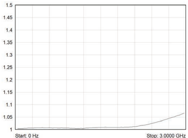
Typical VSWR - 3 GHz Terminated & Unterminated Versions
