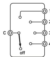
Single Unterminated SP4T
