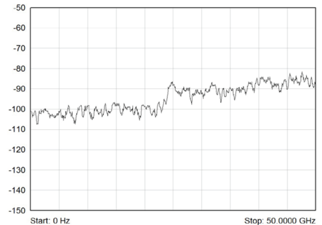
Typical Isolation (dB) - 50 GHz Terminated & Unterminated Versions
