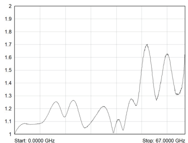
Typical VSWR - 67 GHz Underterminated Versions
