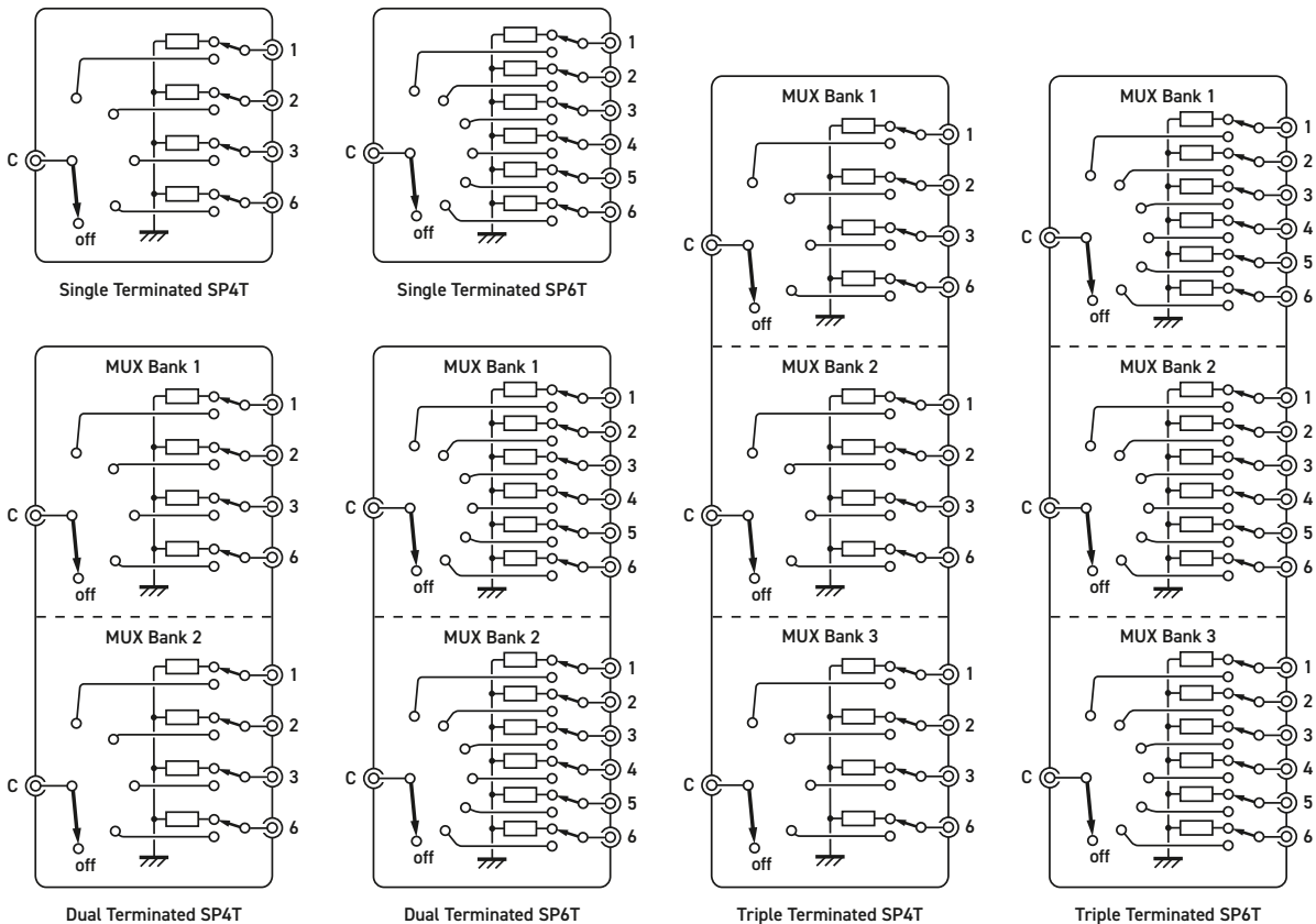
4x-785C Terminated Multiplexer Range (triple versions are only available in remote mount format)
