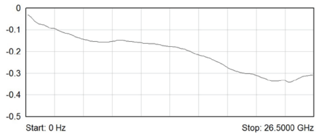
Typical Insertion Loss (dB) - 26.5 GHz Underterminated Versions
