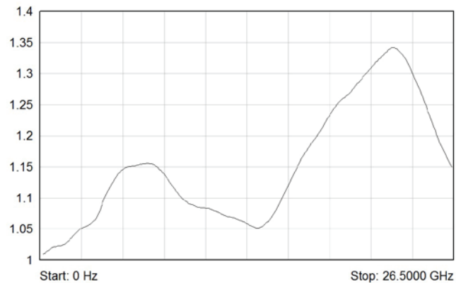
Typical VSWR - 26.5 GHz Underterminated Versions
